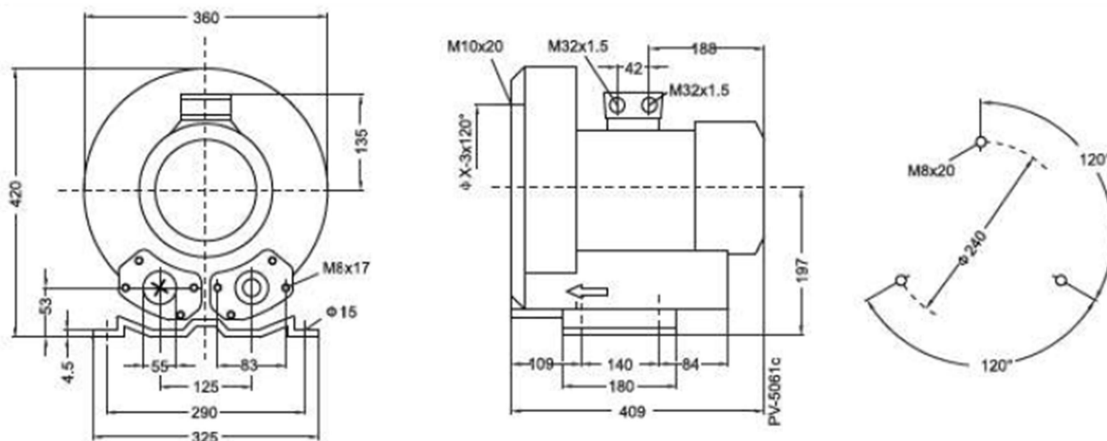
Lajac blower installation drawing
