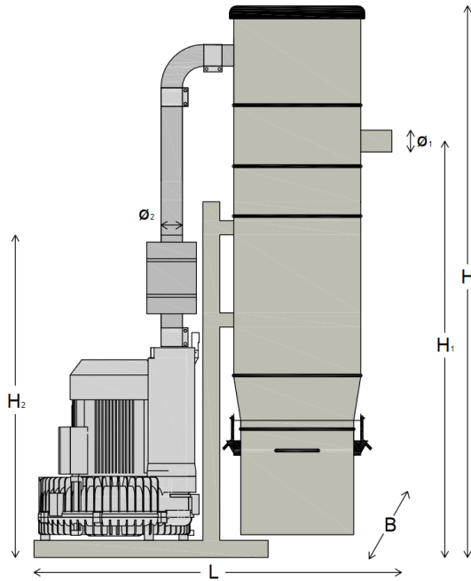
CE-MOB Mobile unit
