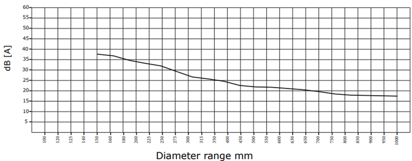
Sound damping silencer length 2000mm
