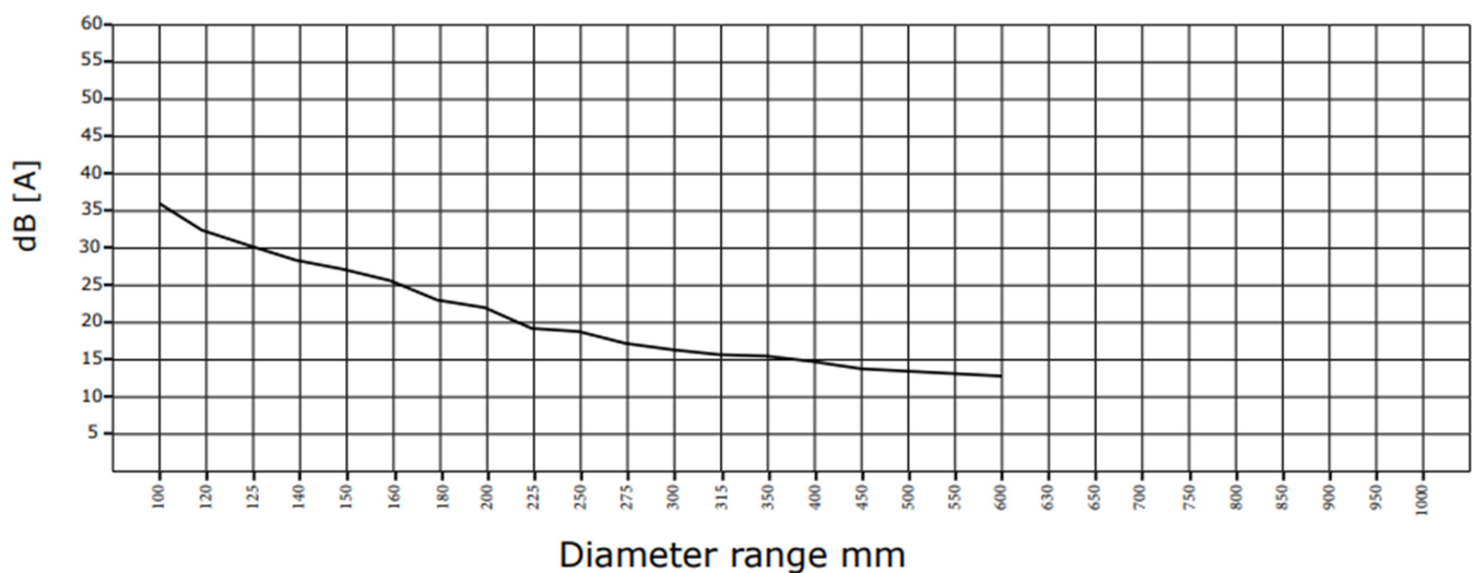
Sound damping silencer length 500mm
