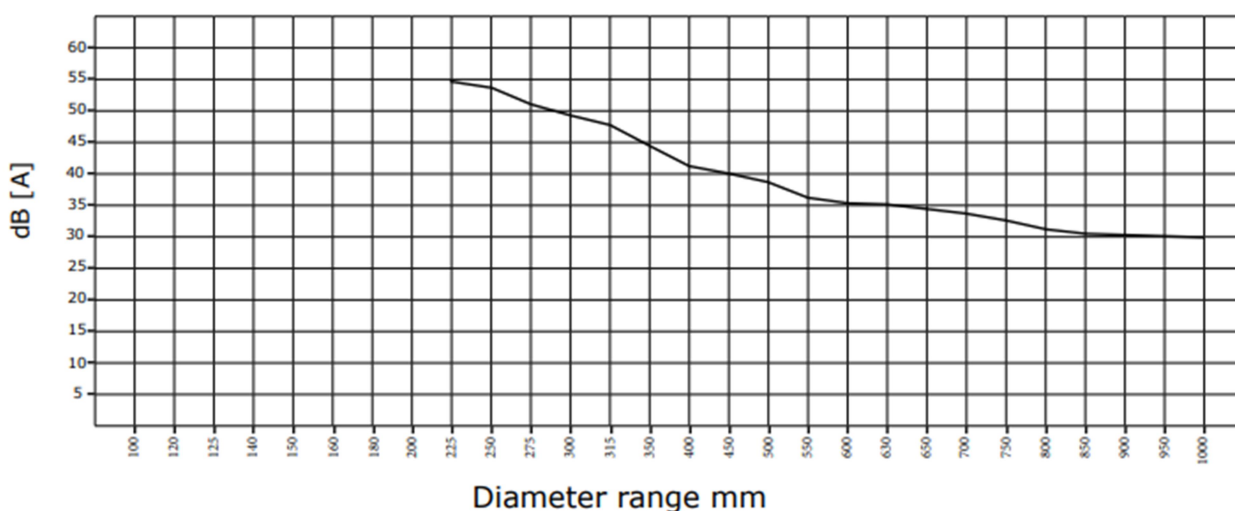
Sound damping silencer length 1000mm
