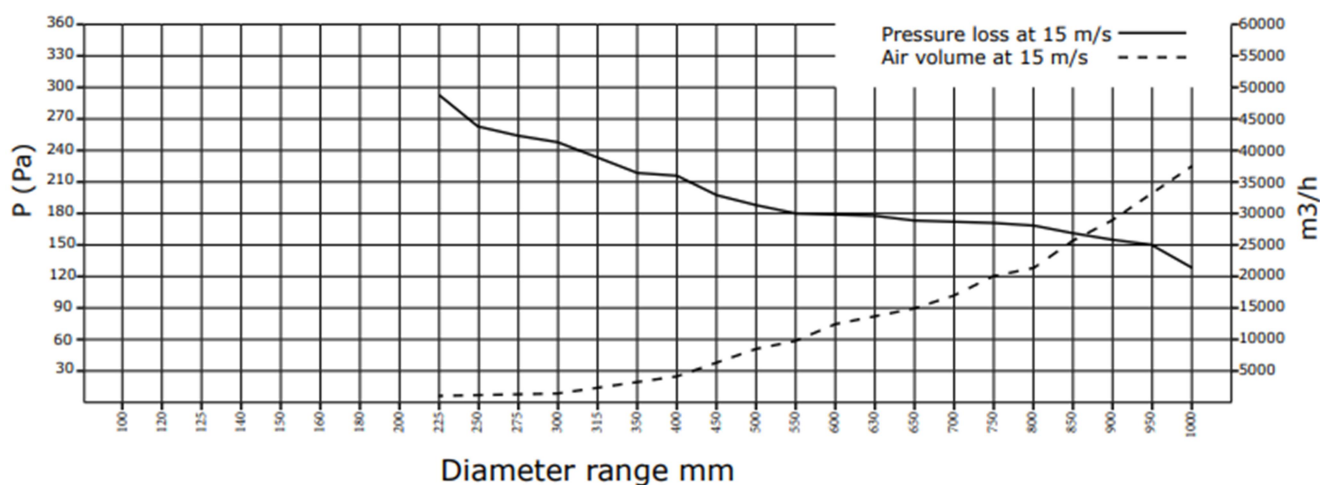
Pressure loss silencer Length 1000mm
