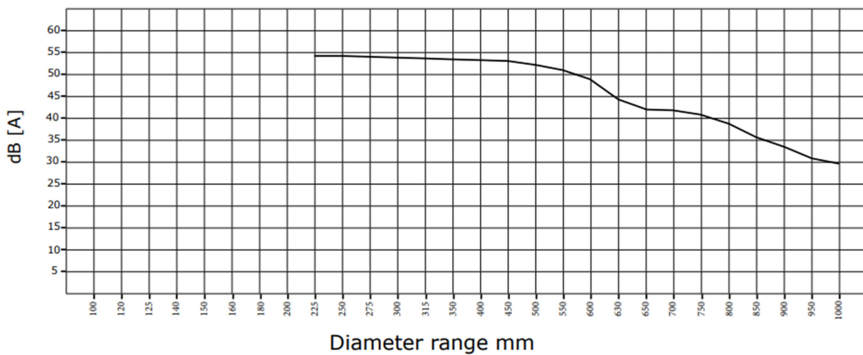
Sound damping silencer length 2000mm
