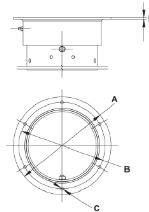
Fume Arm Mounting Flange
